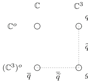
Fig. 1. Krajewski diagram of super-QCD. The nodes represent the representation of \mathbb{C} \oplus M_3(\mathbb{C}) horizontally and of \mathbb{C}^\circ \oplus M_3(\mathbb{C})^\circ vertically. The dotted line indicates how the squark and antisquark appear as components in the (finite) Dirac operator. Note that we do not actually have a copy of \mathbb{C} in the algebra, but see the discussion in the beginning of this subsection
